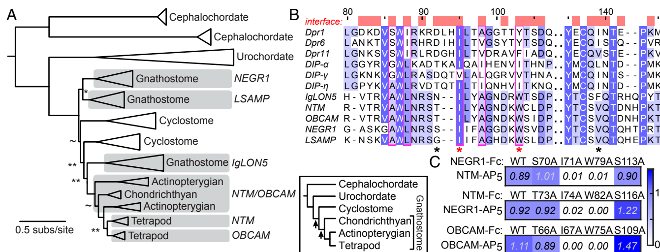
Fig. 2. IgLONs are the vertebrate Wirins. (A) The ML phylogeny of the IgLON subfamily. aLR statistics are shown as branch supports: ** > 9.2 (= 2 In100), * < 4.6 (= 2 In10), ~ < 2.2 (= 2 In3). Unmarked branches have aLR statistics > 9.2. Inset shows the established chordate phylogeny, with arrows marking two genome duplications. (B) Sequence alignment of the IG1 domains of mouse IgLONs, three Dprs, and three DIPs. Amino acids at the Dpr-DIP interface, defined by a 4-Å cutoff from the binding partner, are labeled as red blocks above the alignment. Amino acids mutated in C are labeled with an asterisk. The hydrophobic core residues of the Dpr-DIP interface observed by Cheng et al. (11) is indicated by magenta columns. Sequence numbers above the alignment are for Dpr1. (C) Mutations at the predicted interfaces of the OBCAM-OBCAM and NTM-NEGR1 complexes affect binding as tested using ECIA. To effectively compare WT to mutants, protein concentrations within each mutant series were normalized. Reported absorbance values are after subtraction of negative controls at 0.05 (±0.01) absorbance units.
