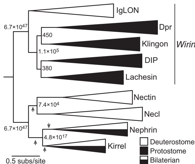
Fig. 1. The ML phylogeny of the Wirin family. Branch labels indicate approximate likelihood ratios (aLRs), defined as the likelihood of the ML topology divided by the likelihood of the next-best rearrangement of branches around the given branch. Arrows indicate alternative rootings that entail the same number of gene gains and losses as the phylogeny shown. For unreduced phylogenies, see Datasets S1–S6 .
